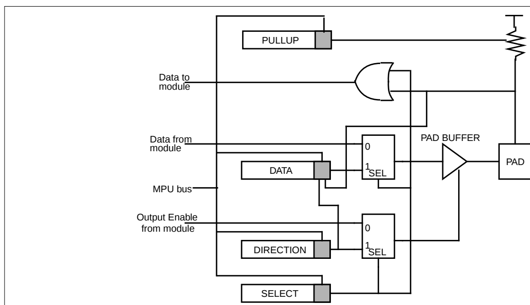
Figure 7-2. Pullup Port
