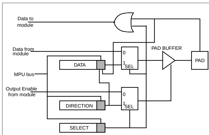
Figure 7-1. Basic Port
