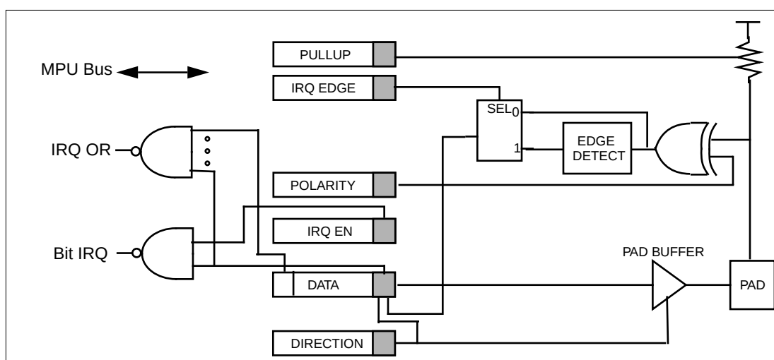
Figure 7-3. Interrupt Port
