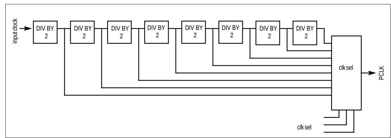
Figure 11-3. PWM Prescaler
