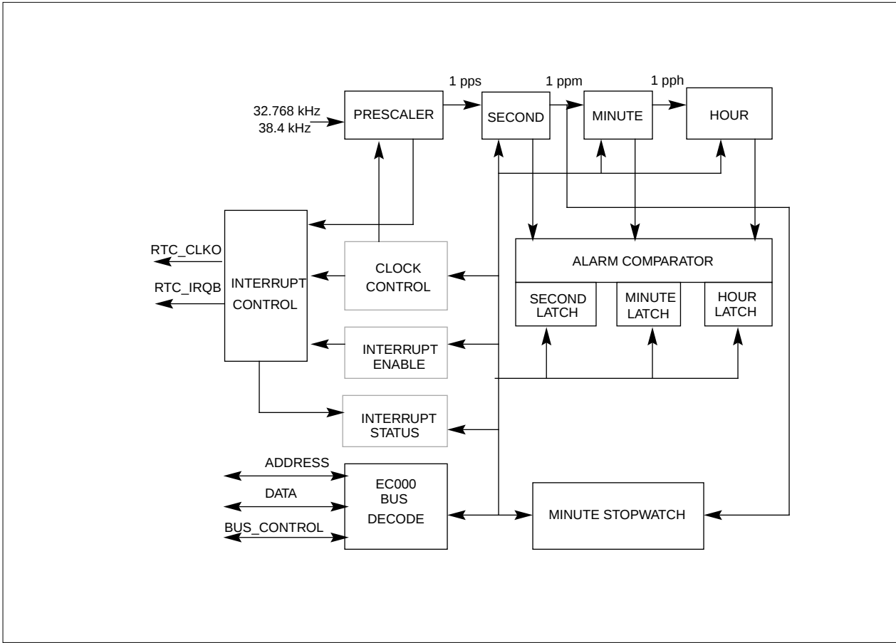
Figure 5-1. Real-Time Clock
