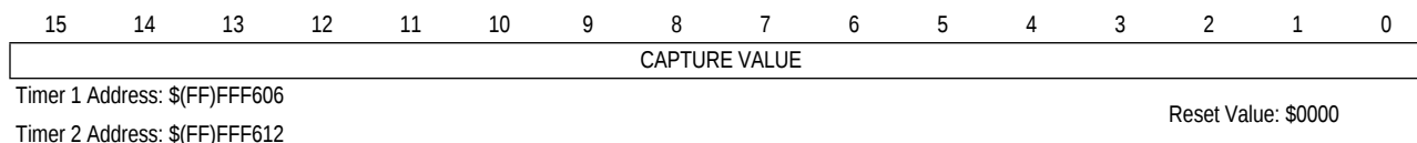
Figure 6-7. Timer-Capture Register
