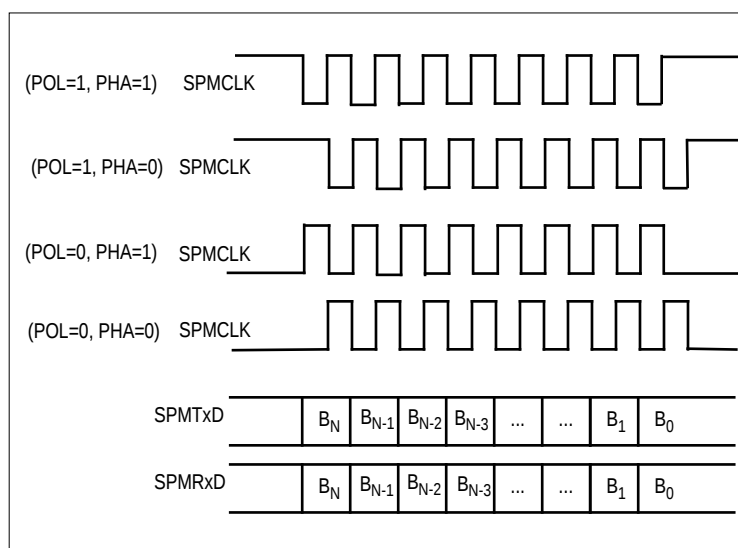
Figure 10-2. Master SPI Operation
