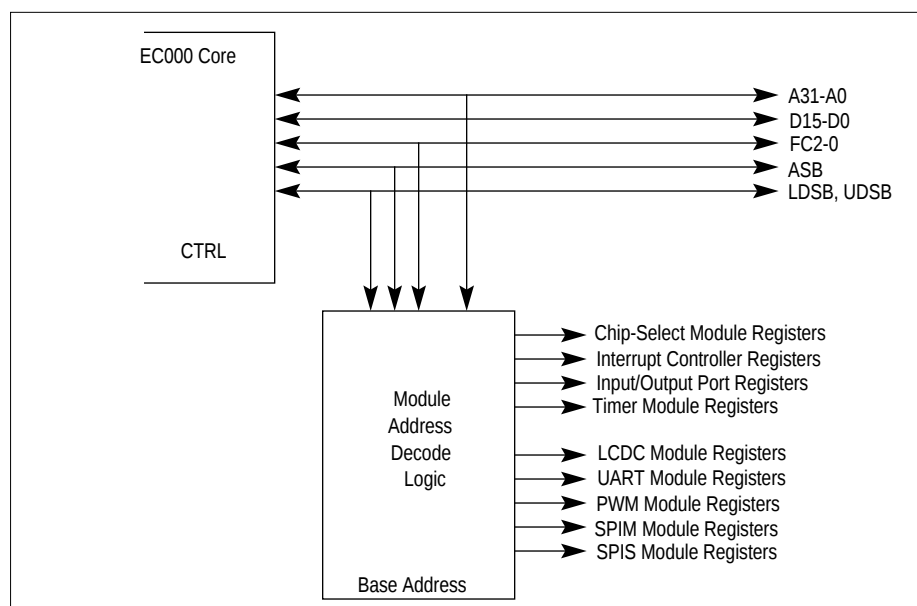
Figure 2-1. Chip-Select Logic
