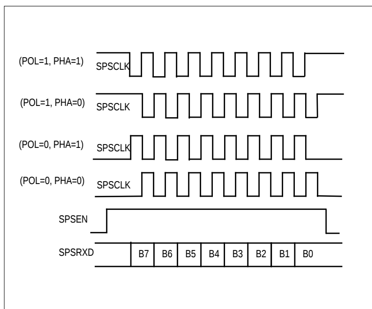
Figure 9-2. SPIS Operation
