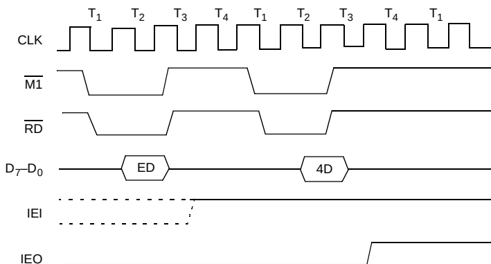
Figure 12. Return from Interrupt Cycle
