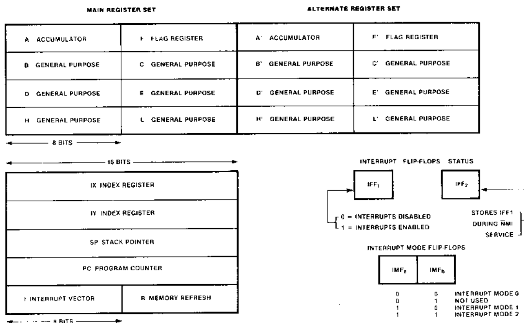
Figure 4. CPU Registers
