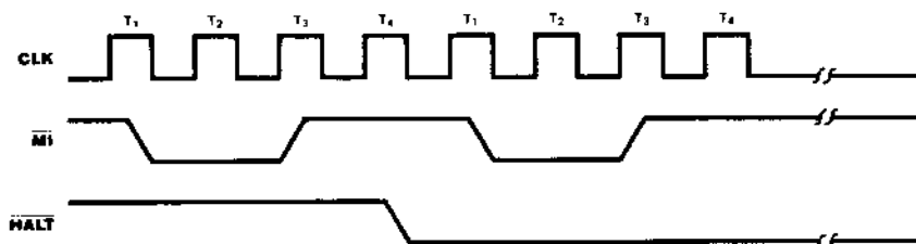
Figure 13. Power-Down Acknowledge
