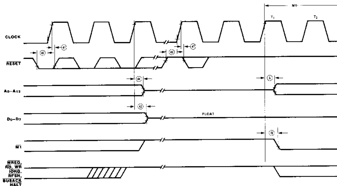
Figure 12. Reset Cycle
